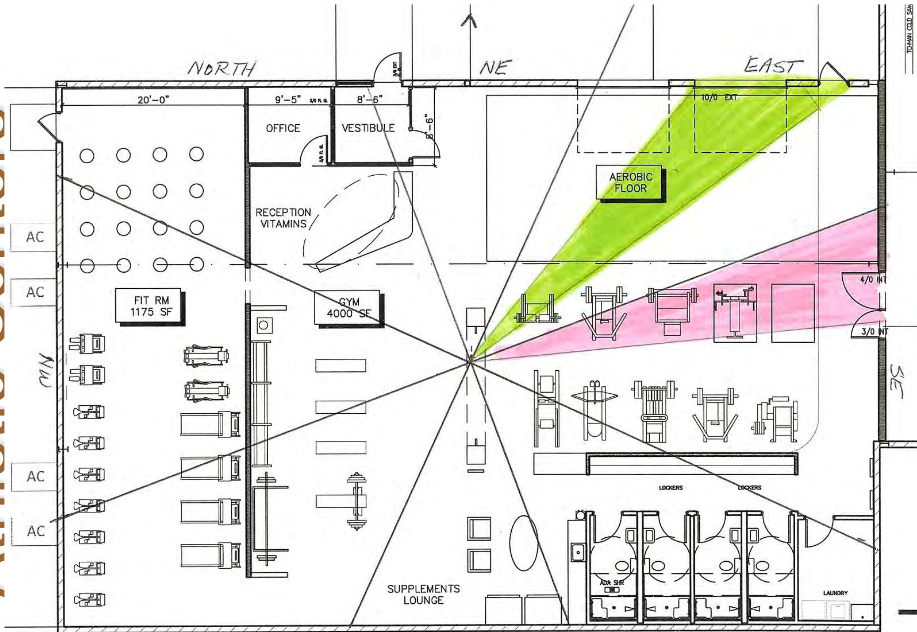
1 PARTIAL FLOOR PLAN 1/8" = 1'-0"
